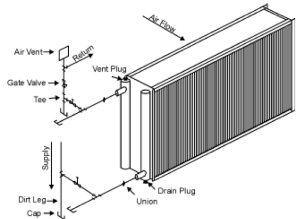
Figure 4: Horizontal Air Flow
