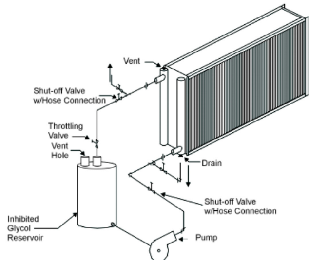
Figure 8: Flushing System
